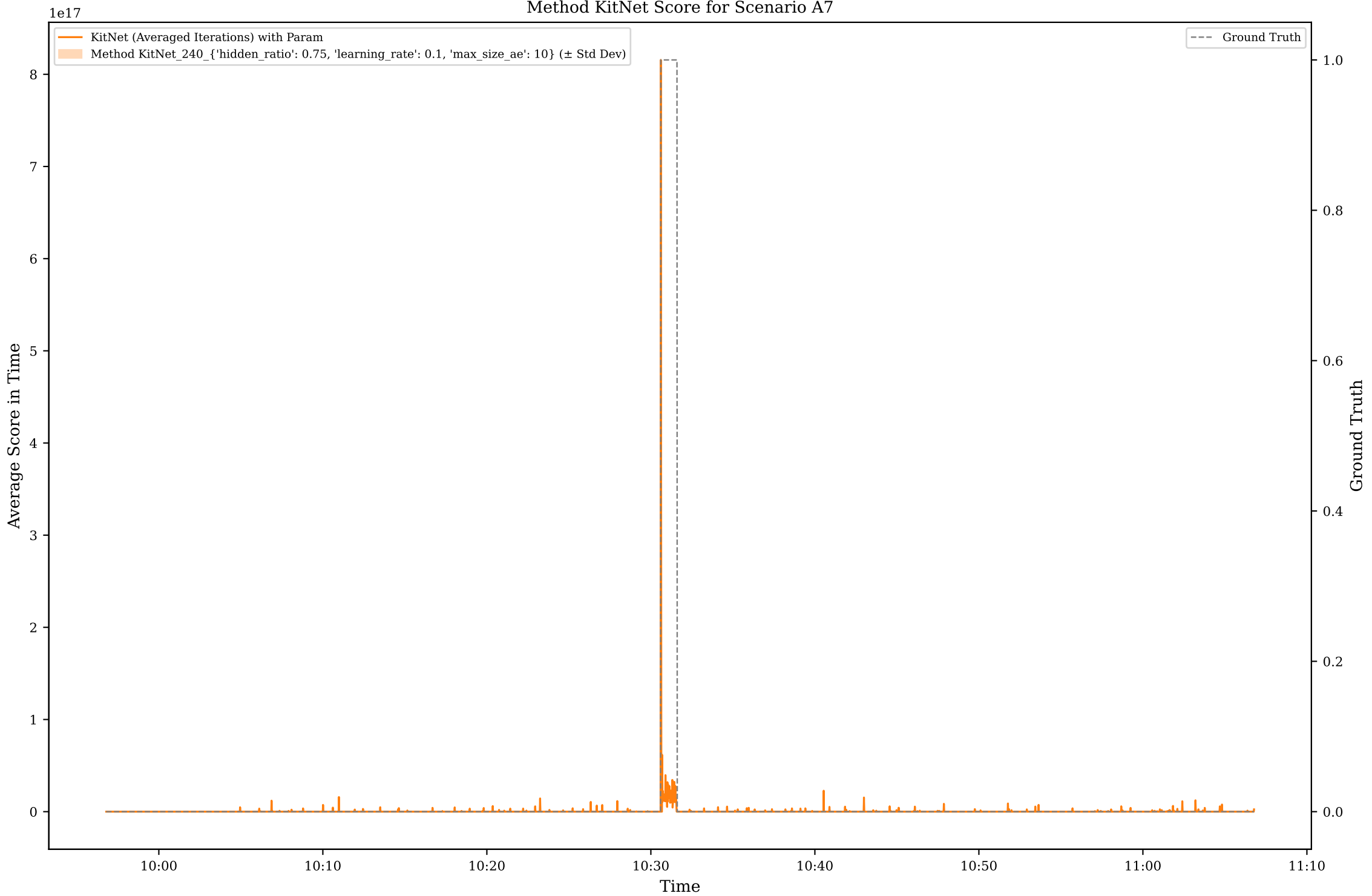
Method KitNet Score for Scenario A7
